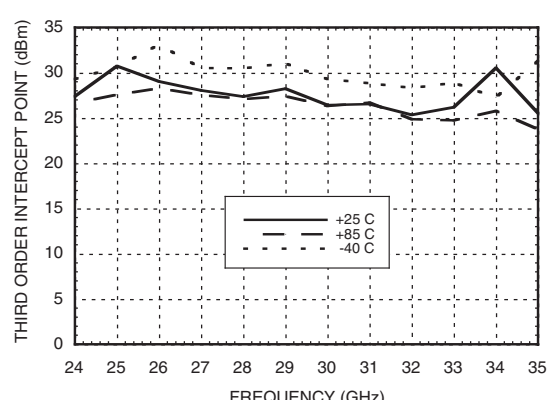
Output IP3 vs. Temperature @ Vdd = +6V
